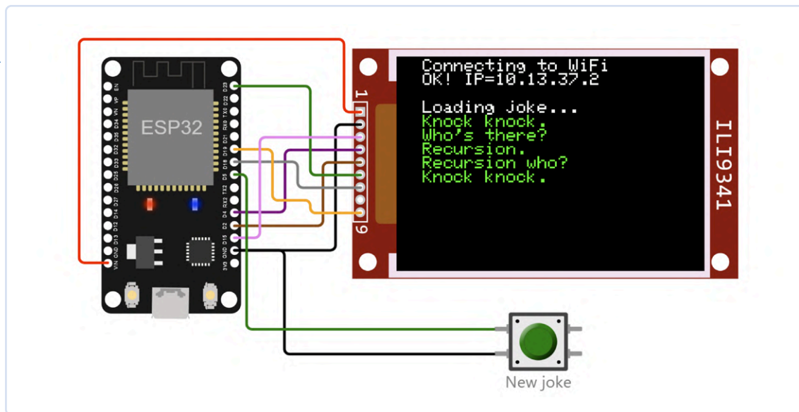
Figure 2: Wi-Fi Simulation Client example [8].
