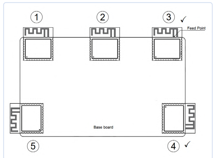
Figure 4: Positioning a module on a base board. (Source [6])
