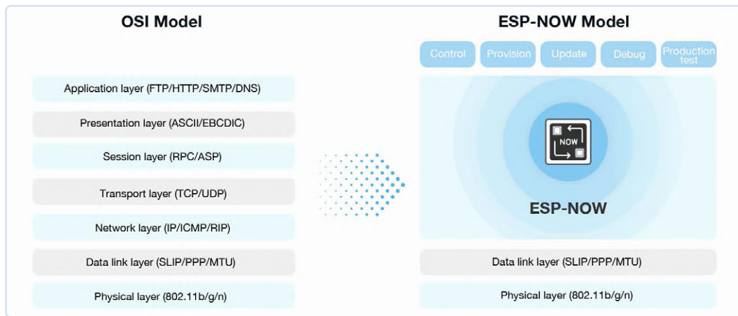
Figure 2: The ESP-NOW Model simplifies the top five layers of an OSI Model into one layer.
