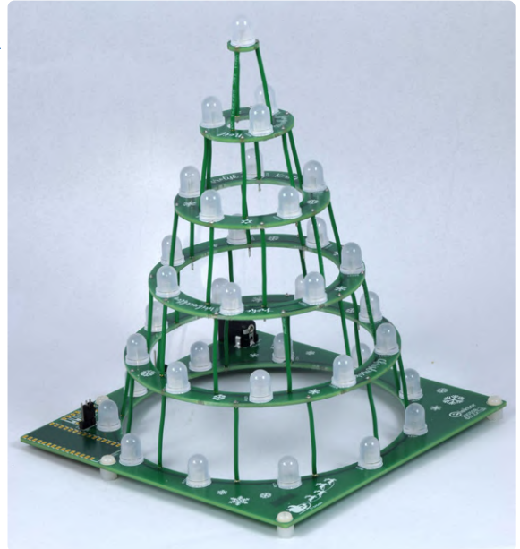
Figure 5: The completed prototype, without the optional Arduino module.
