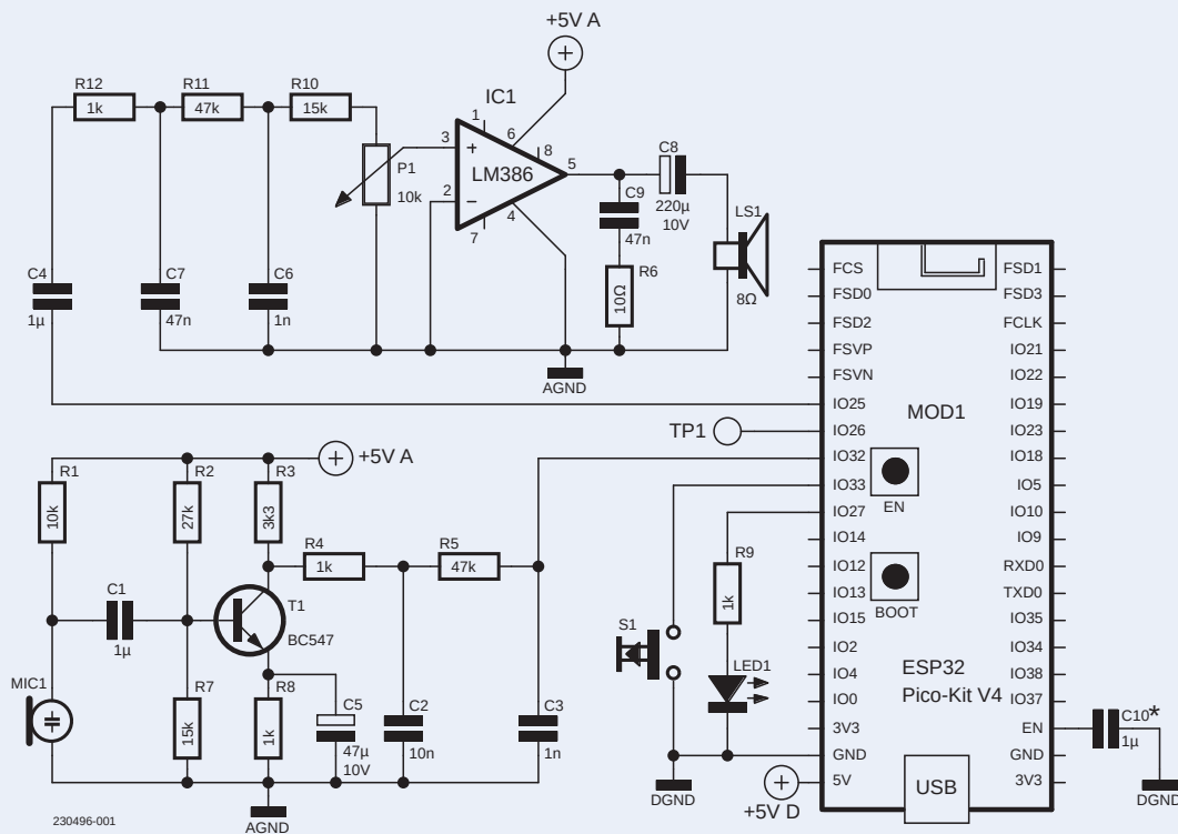
Figure 3: A simple microphone preamplifier on the input and a classic LM386 as power amplifier at the output. Note how the power supplies for the analog and digital parts are separated.
