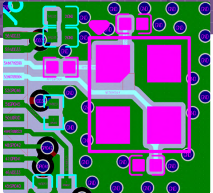
Figure 3: The two load capacitors should be placed on two sides of the crystal.
