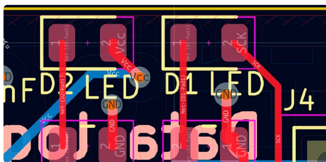
Figure 4: Pads without teardrops (left) and with added teardrops (right).
