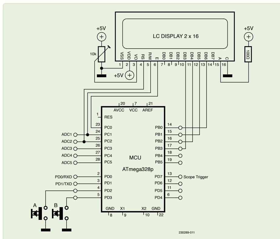
Figure 4: Schematic for Test & Demo application with an ATmega328P.
