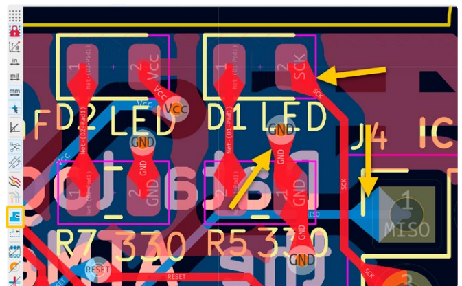
Figure 4: Pads without teardrops (left) and with added teardrops (right).
