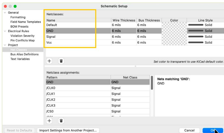
Figure 6: Net classes and their net assignments are now integrated across the schematic and PCB editors. Here, you can see the existing netclasses in the schematic editor.
