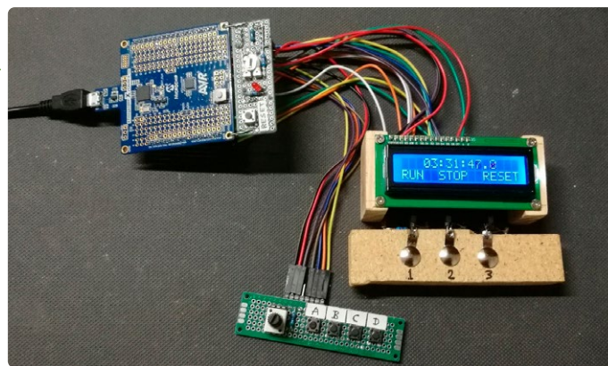
Figure 3: Test & Demo Setup with AVR X-mini board.
