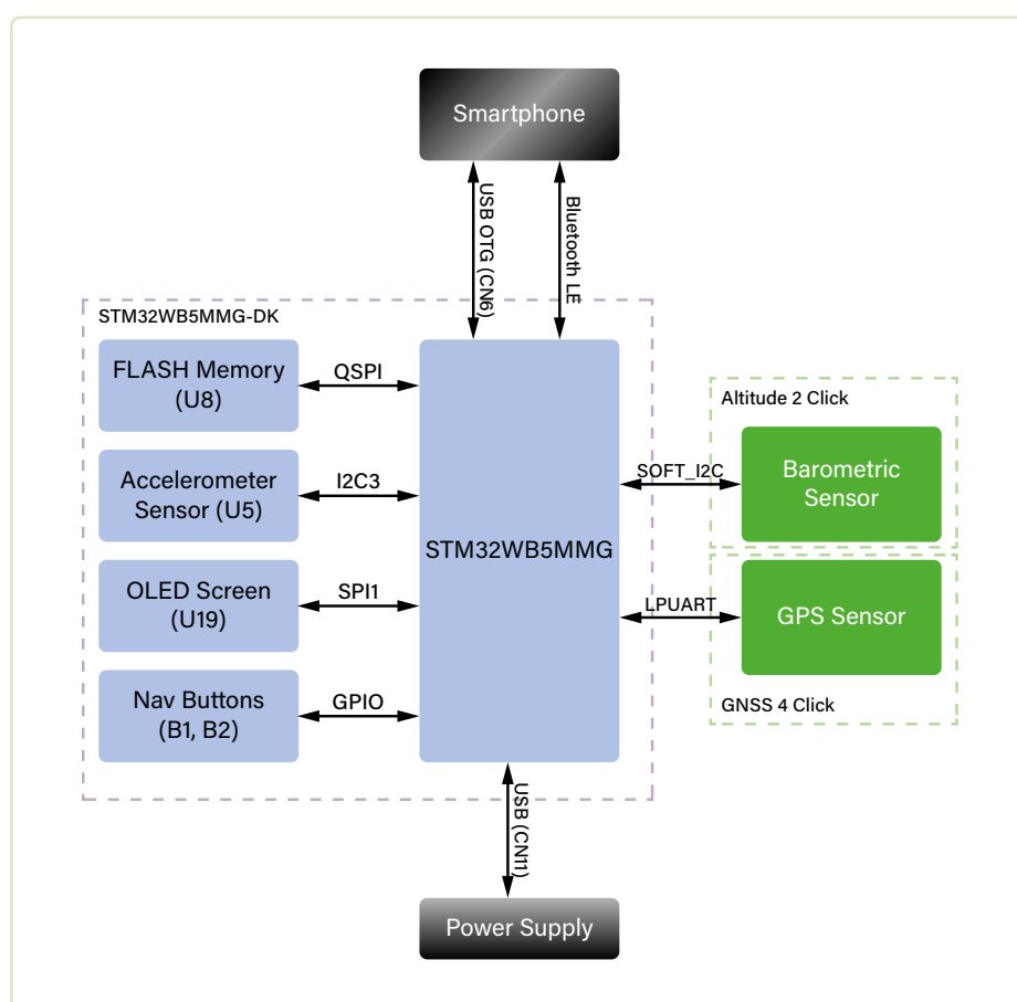
Figure 2: Functional block diagram of the system, showing the physical interfaces to the external modules.
