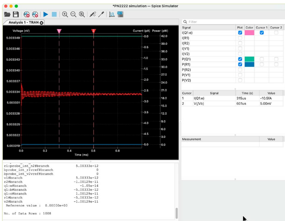
Figure 9: A transient simulation plot in the updated KiCad circuit simulator.
