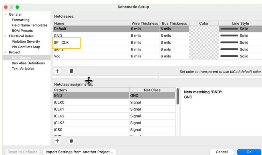
Figure 8: The new net class has been synced in the schematic editor.
