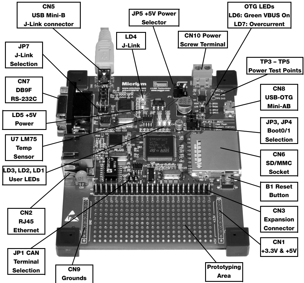
Figure E-3 μC/Eval-STM32F107 Board Layout
