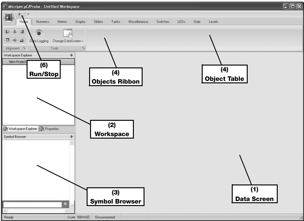
Figure D-2 Empty \mu C/Probe project
