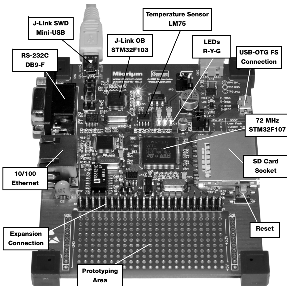
Figure 1-1 Micrium's \mu C/Eval-STM32F107
