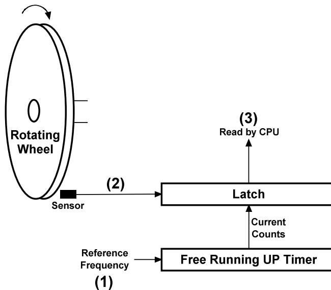
Figure 7-6 Using an Input Capture to measure RPM
