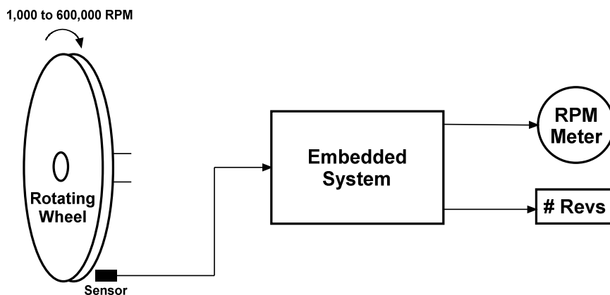
Figure 7-1 RPM Measurement
