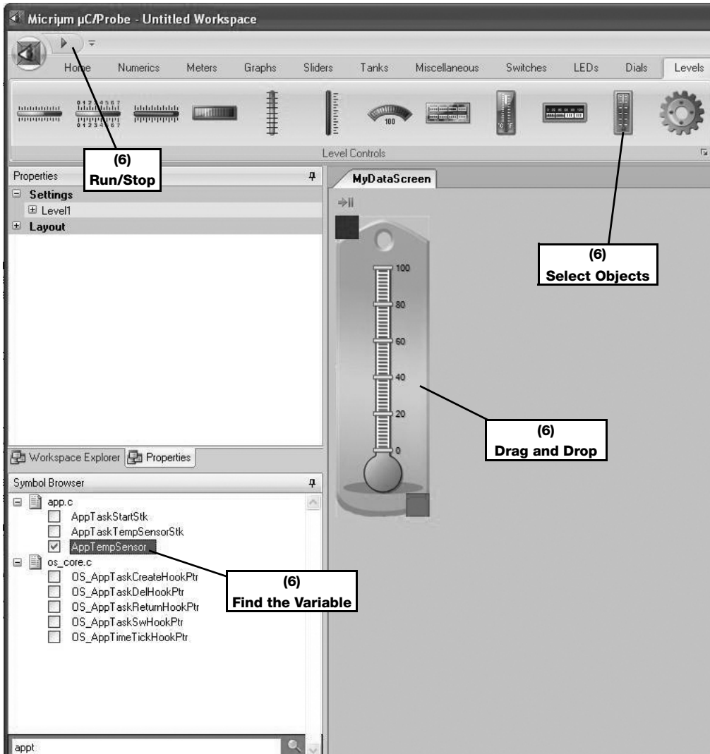
Figure D-6 Assigning a variable to an object
