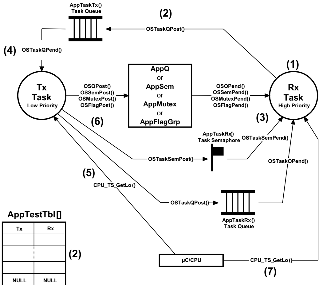
Figure 6-3 Signal Semaphore
