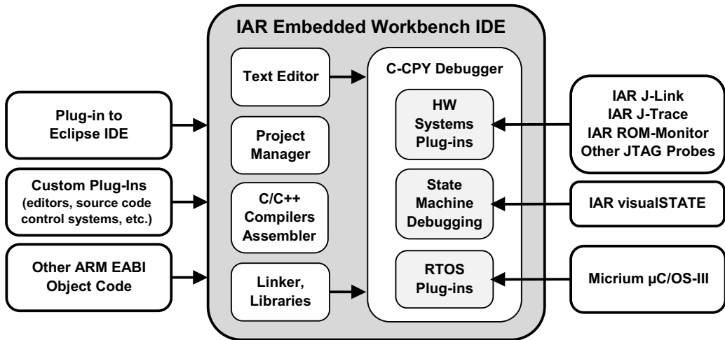
Figure C-1 IAR Embedded Workbench
