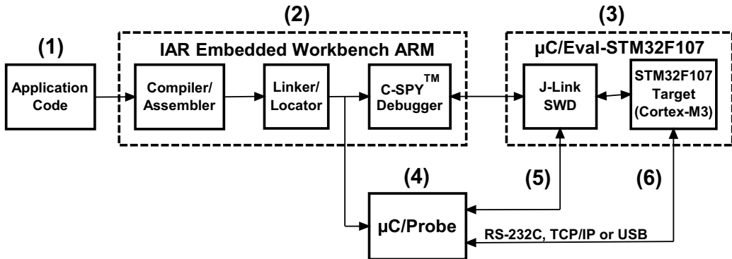
Figure D-1 Development environment using the \mu C/Eval-STM32F107
