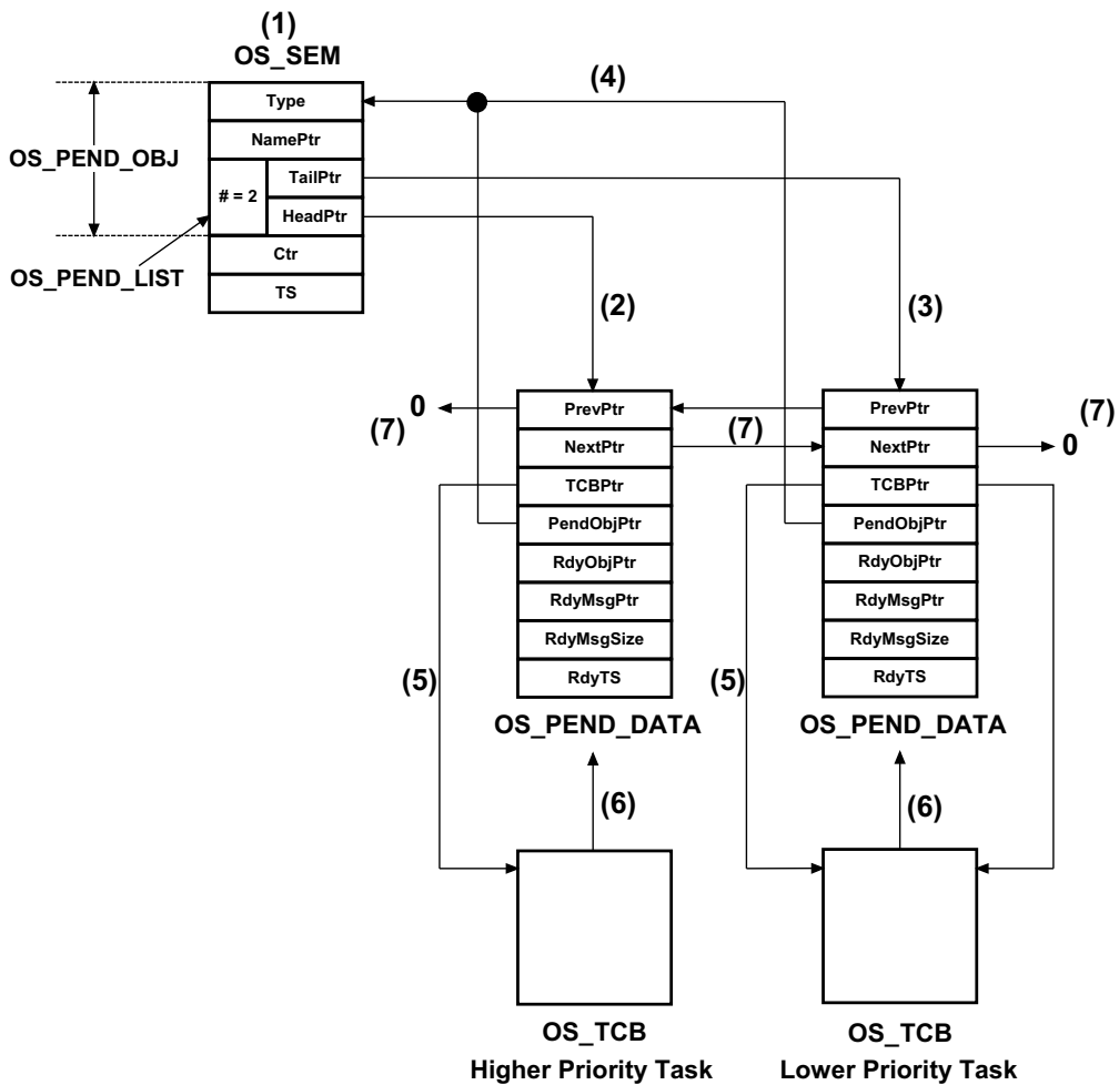
Figure 10-4 Pend Data
