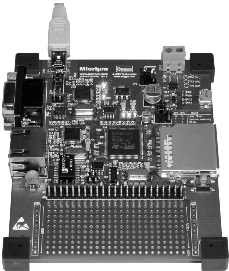
Figure 4-1 μC/Eval-STM32F107 Evaluation Board
