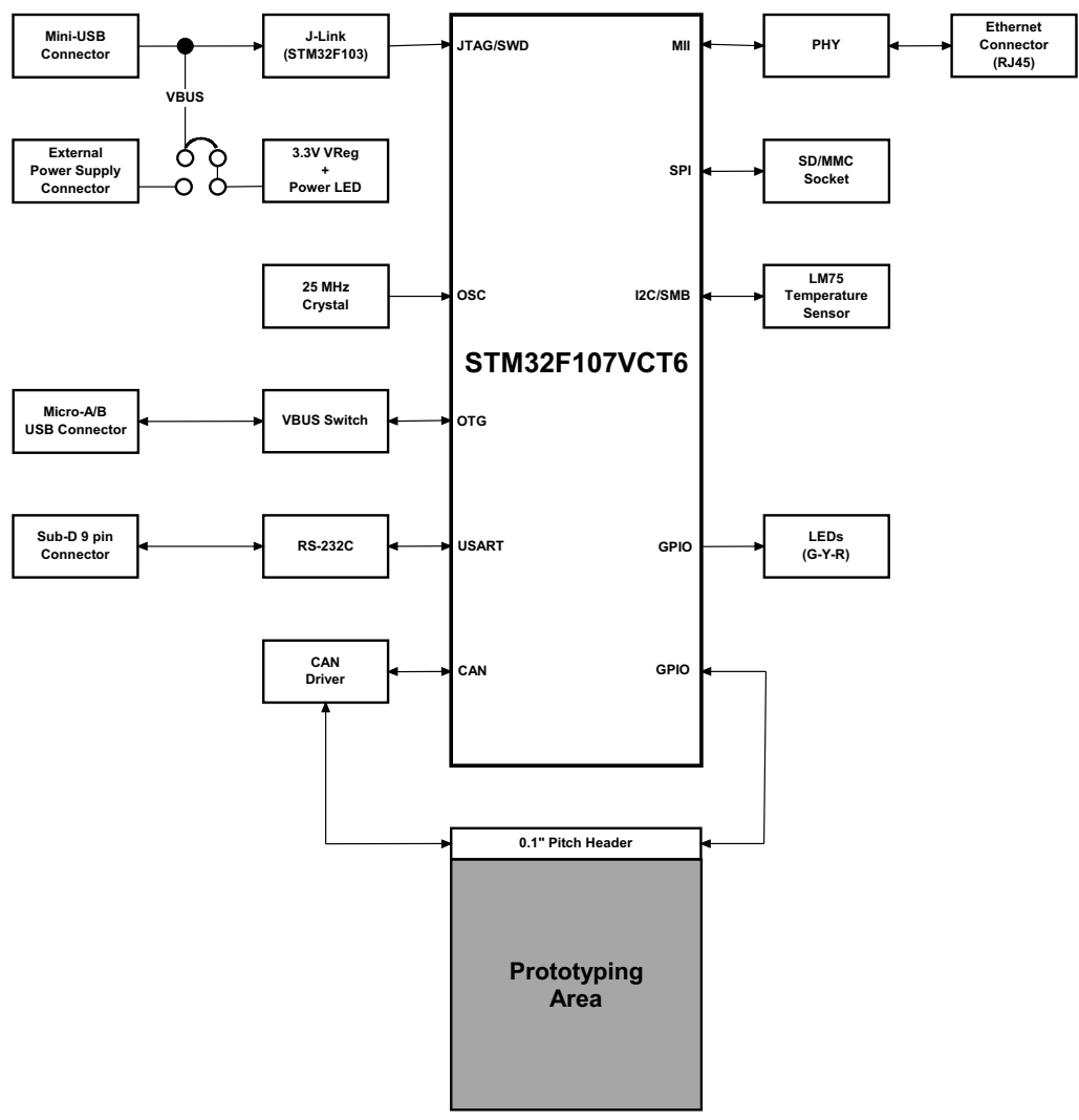
Figure E-2 \mu C/Eval-STM32F107 Hardware Block Diagram
