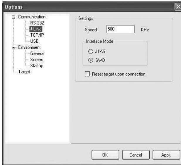
Figure 4-11 μC/Probe's J-Link options
