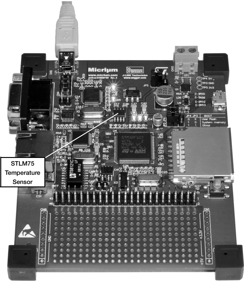
Figure 5-1 μC/Eval-STM32F107 Evaluation Board
