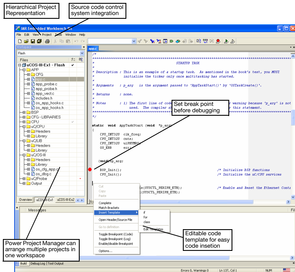
Figure C-2 IAR Embedded Workbench IDE
