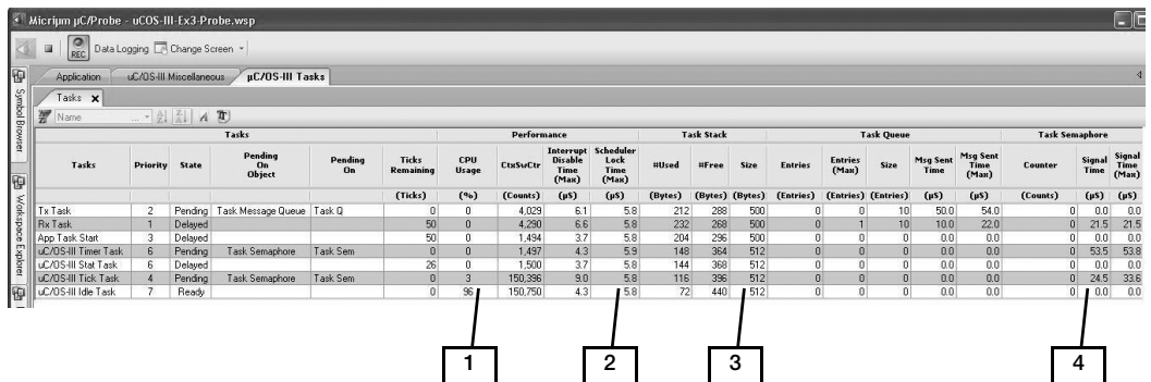
Figure 6-4 μC/OS-III Task Screen
