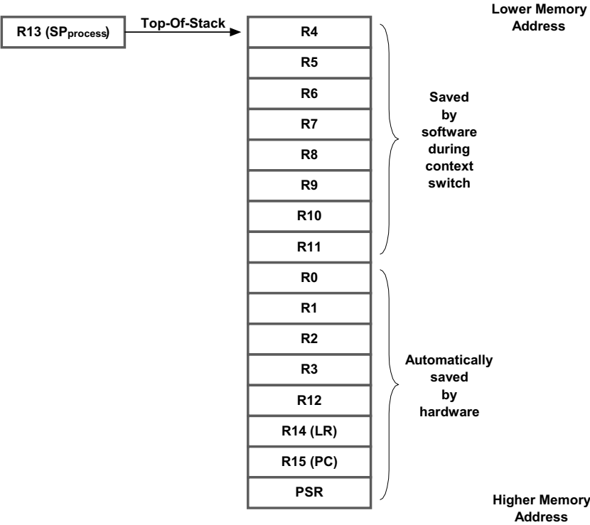
Figure 2-3 Cortex-M3 Register Stacking Order
