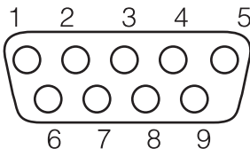
Figure E-4 μC/Eval-STM32F107 DB-9F RS-232C connector CN6 with ISP support (front view)
