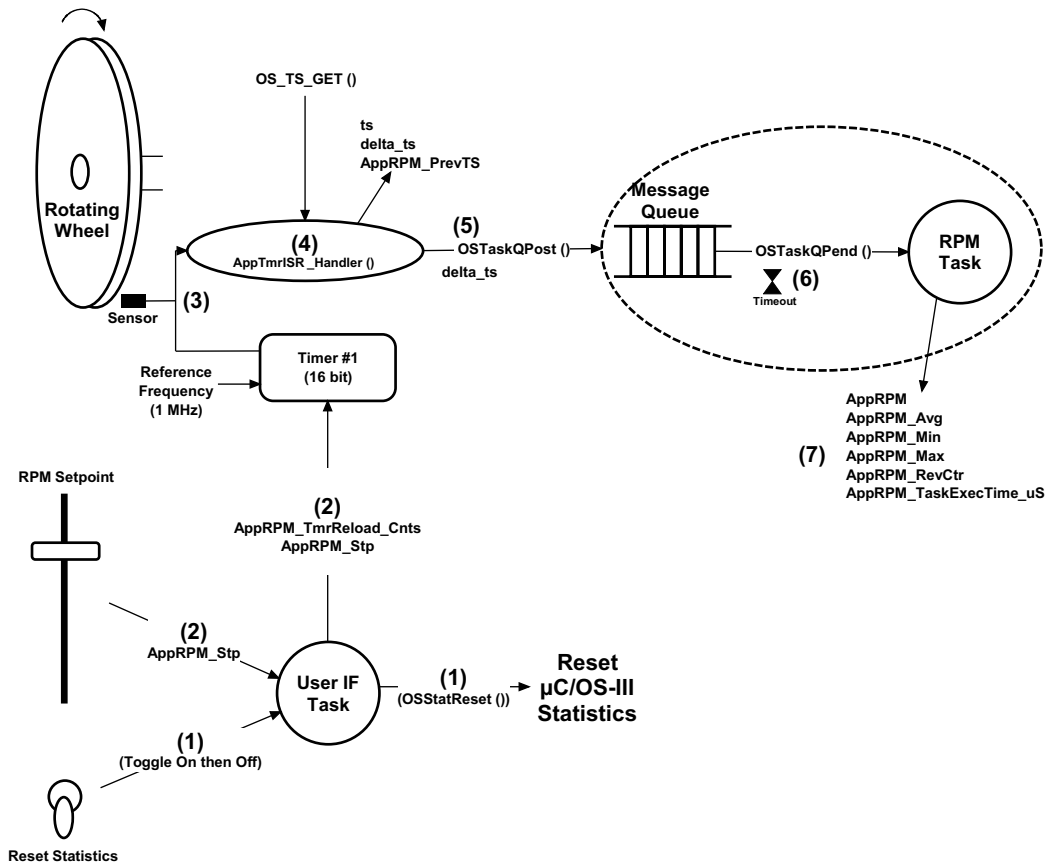
Figure 7-5 Measuring and computing RPM
