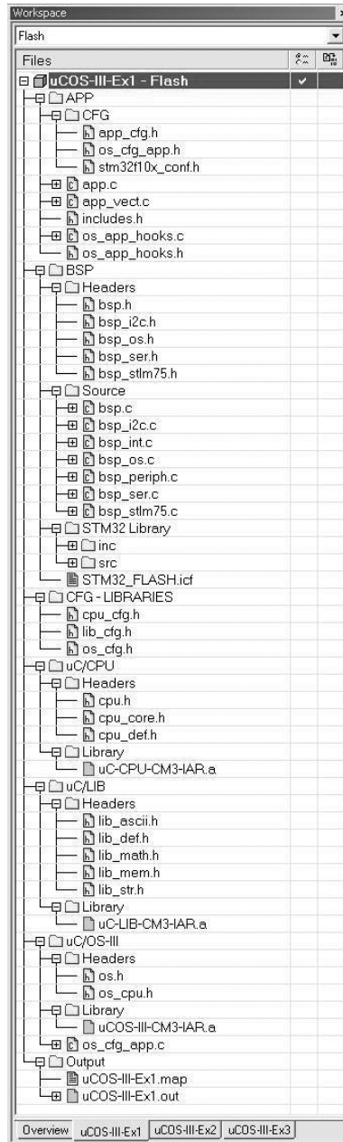
Figure 4-3 Expanded Workspace for uCOS-III-Ex1
