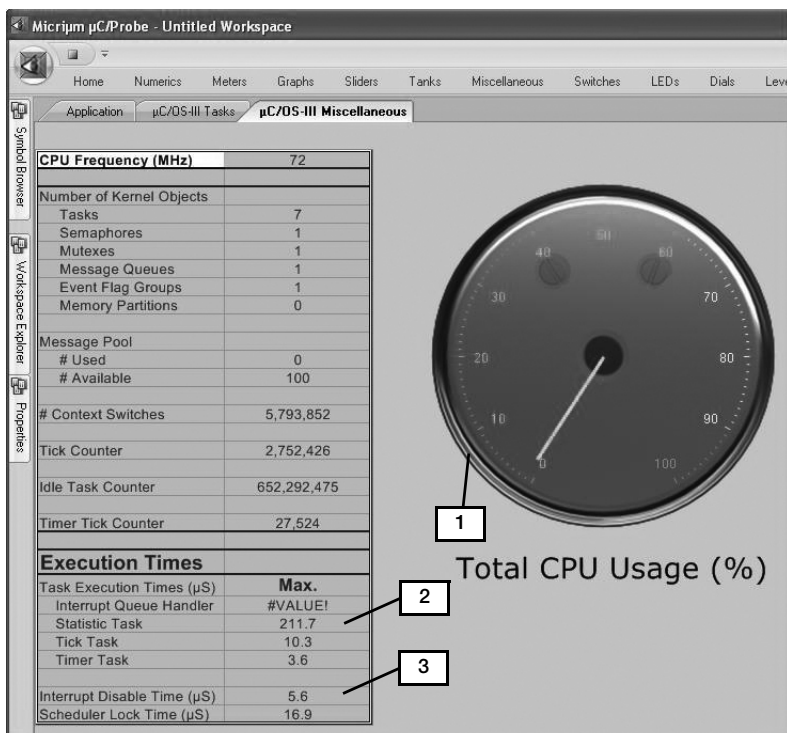
Figure 6-5 μC/OS-III Miscellaneous Screen
