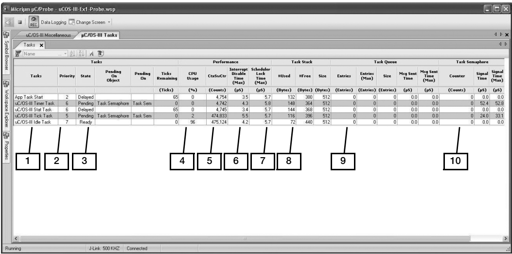
Figure 4-13 μC/Probe Example #1 Run Mode Screen
