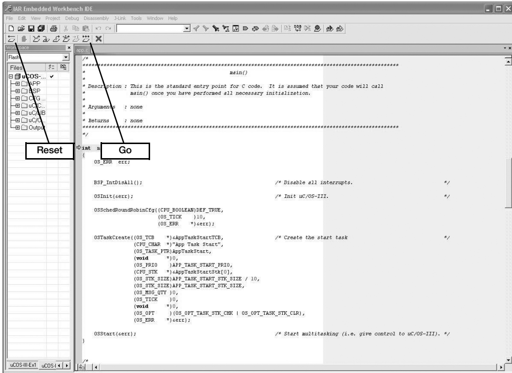
Figure 5-3 Stops at main() after code is downloaded
