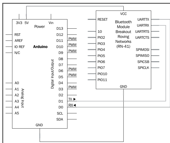
The corresponding circuit diagram is as follows:
